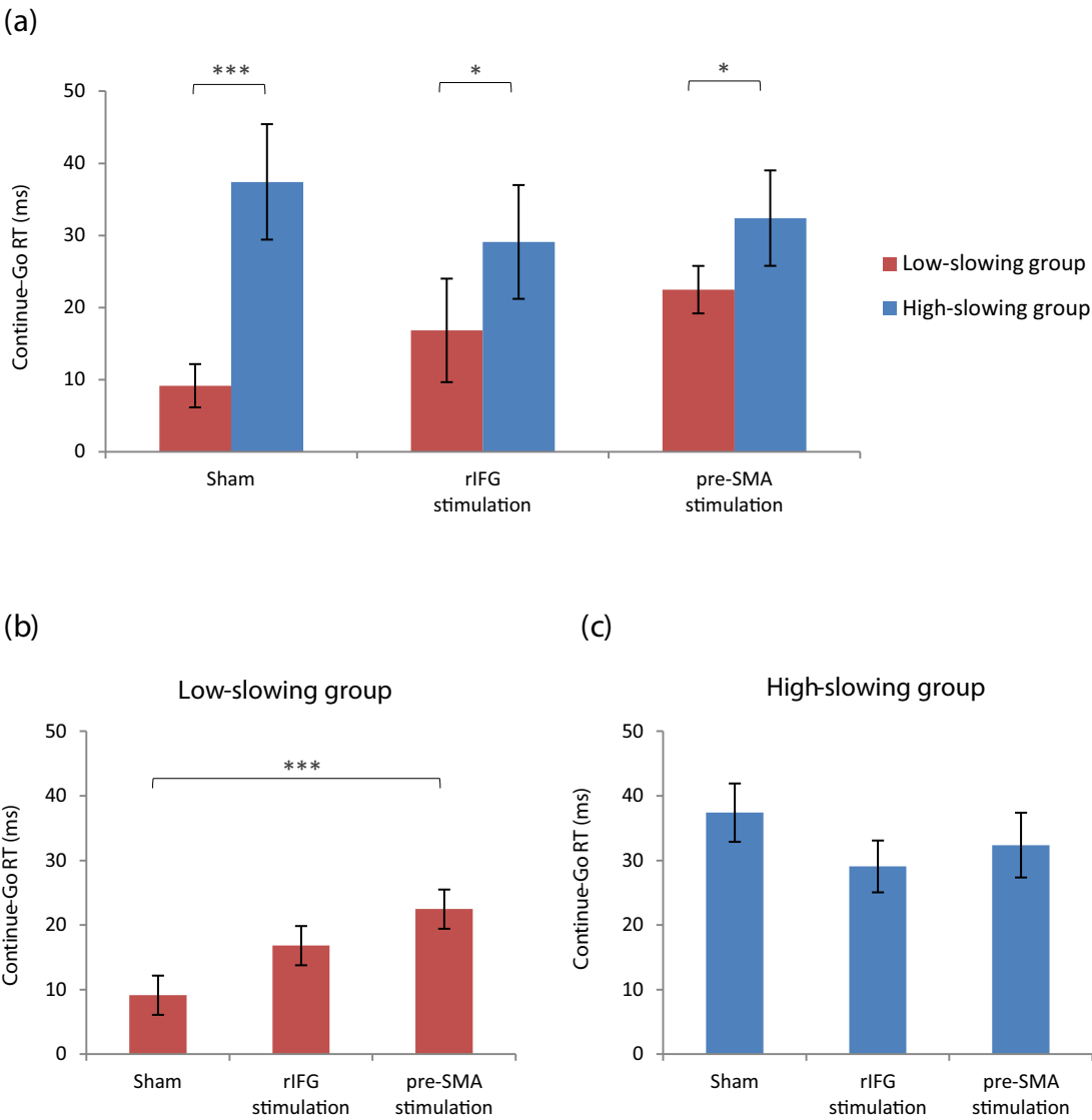
Fig. 3. Panel (a) shows the between-group comparison in the three TMS conditions. Error bars denote 95% confidence intervals. Panels (b) and (c) show the within-group differences in continue–go RT for the low- and high-slowing groups in the three TMS conditions. Applying TMS over the right pre-SMA significantly increased the low-slowing group's continue–go RT (i.e., their degree of slowing) relative to the sham condition ( p < 0.001 ). Error bars denote 95% within-subjects confidence intervals computed in accordance with Cousineau [12].
