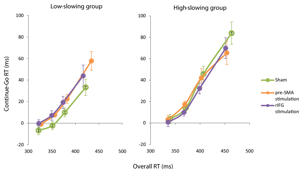
Fig. 4. Delta plots showing the within-group differences in continue-go RT for the low- and high-slowing groups in the three TMS conditions. Error bars denote 95% within-subjects confidence intervals computed in accordance with Cousineau [12].
